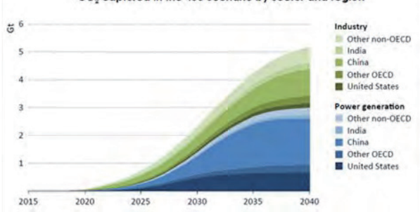
CO 2 captured in the 450 Scenario by sector and region
